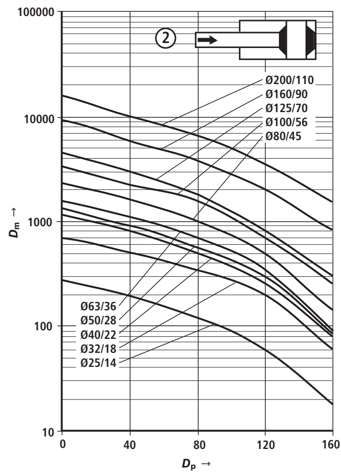
Damping capacity: Retraction and extension with k_v ②
