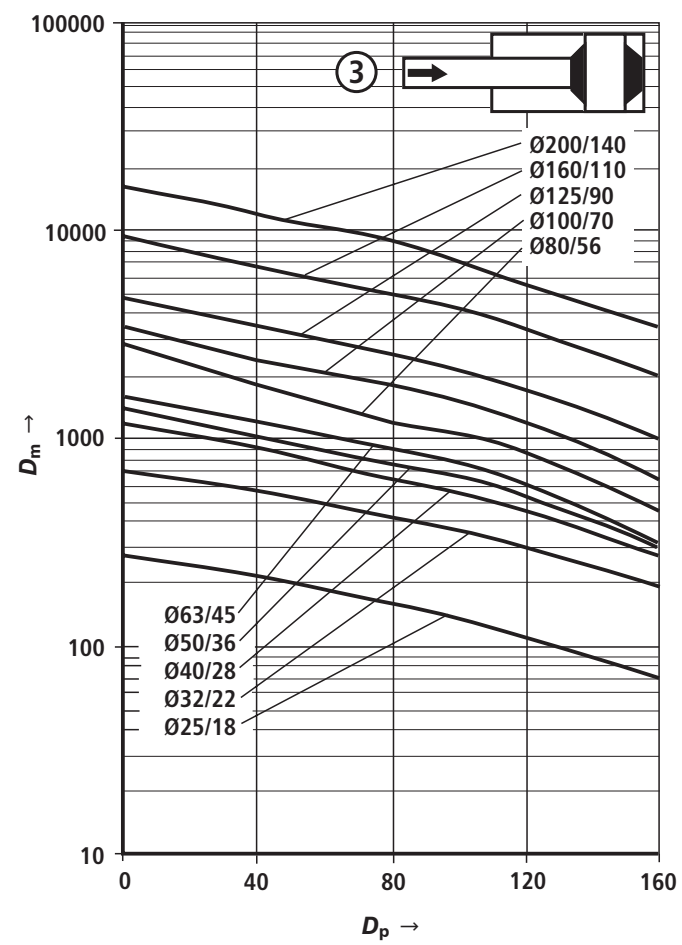
Damping capacity: Retraction and extension with k_v ③
