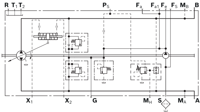
▼ Circuit diagram, standard version 1)
