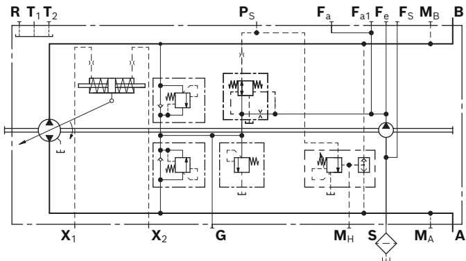
▼ Circuit diagram, version with DA control valve 1)
