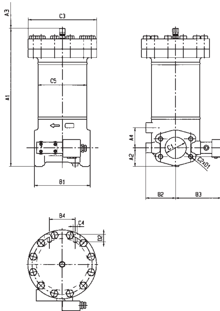
Filter housing for filter elements in accordance with DIN 24550
