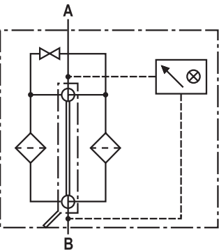
Duplex filter without by-pass valve and with mechanical indicator as well as pressure equalization line
