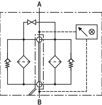
Duplex filter with by-pass valve and mechanical indicator as well as pressure equalization line
