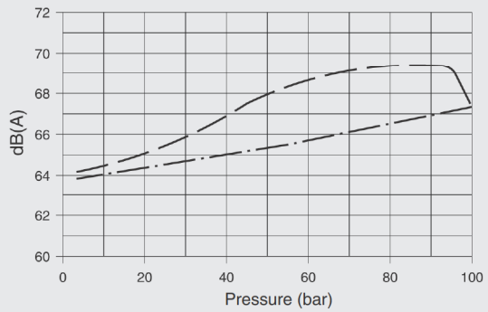
Maximum noise level with sound-level meter placed 1 meter away from pump, flexible coupling PVV101-2-31 / -40 / -50
