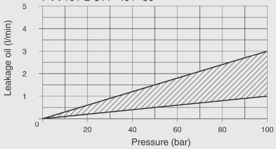
Leakage oil Values determined with pump on zero flow setting PVV101-2-31 / -40 / -50
