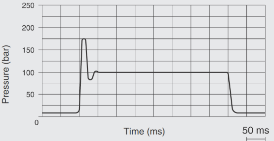
Response times and peak pressure PVV101-2-31 / -40 / -50
